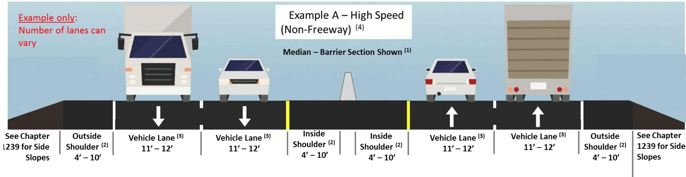
Exhibit 1231-2 Motor Vehicle Oriented Cross Sections
