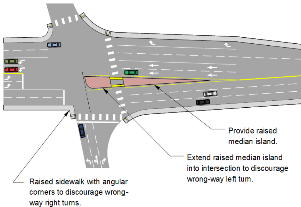
Exhibit 1310-5 Diamond Interchange with Advance Storage
