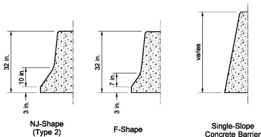
Exhibit 1610-17 Concrete Barrier Shapes
