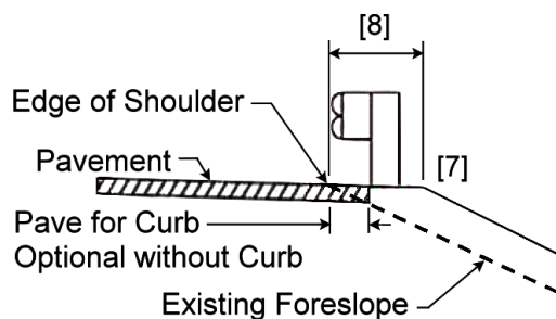
Shoulder Widening for Guardrail
