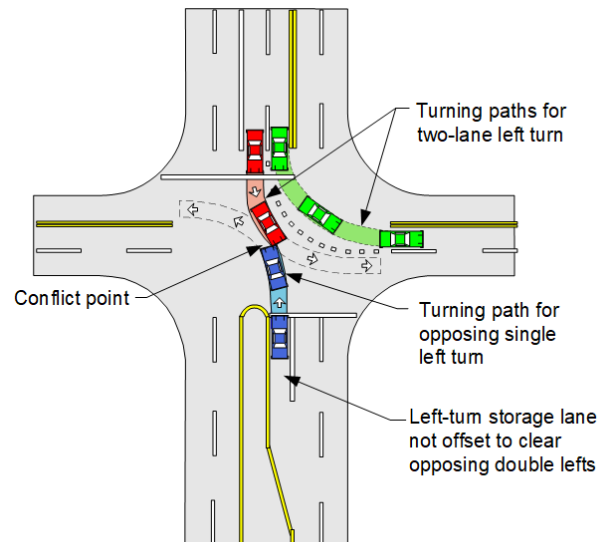
Left-Turn Lane Configuration Preventing Concurrent Phasing
