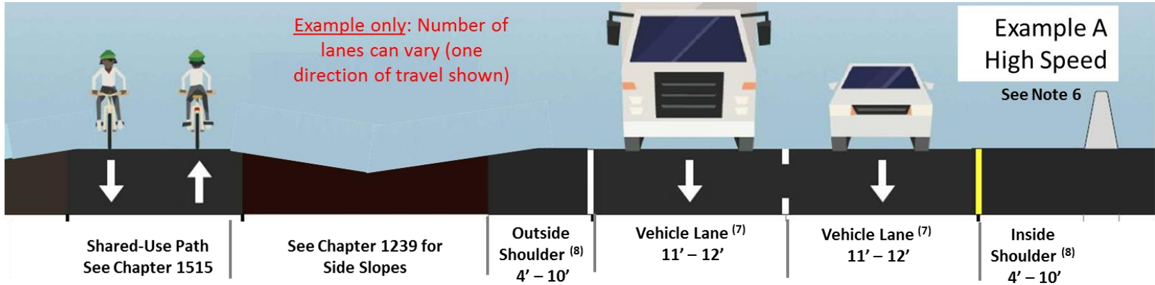
Exhibit 1231-6 Complete Street Cross Sections
