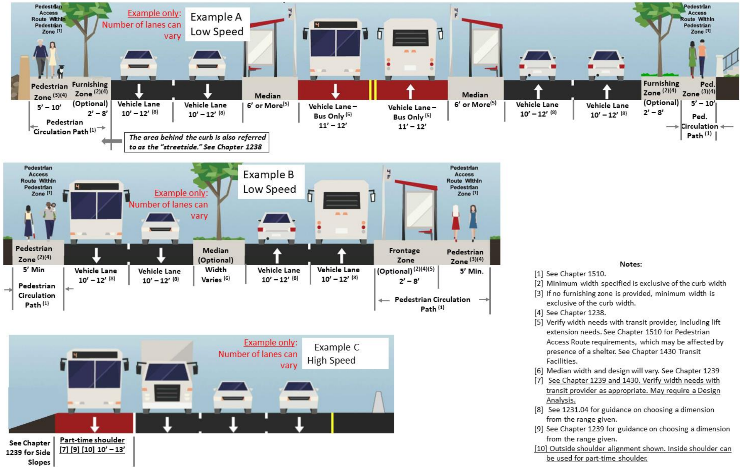
Exhibit 1231-5 Cross Sections Featuring Transit Facilities
