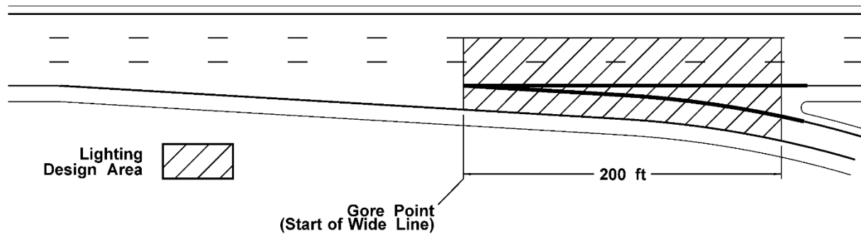
Exhibit 1040-18 Single Lane Off-Ramp Lighting Design Area
