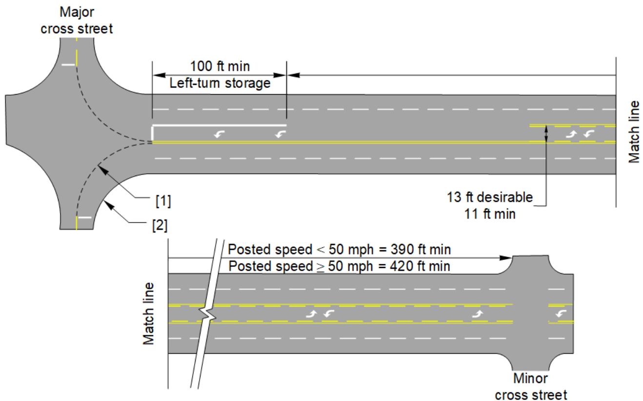
Exhibit 1310-18 Median Channelization: Two-Way Left-Turn Lane
