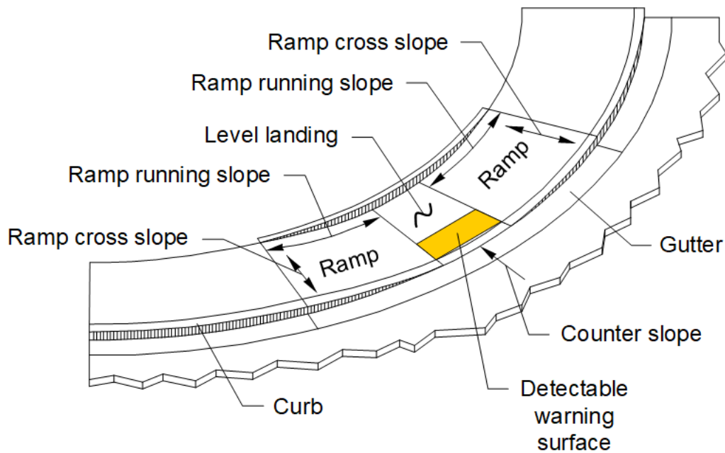
Exhibit 1510-12 Parallel Curb Ramp Common Elements
