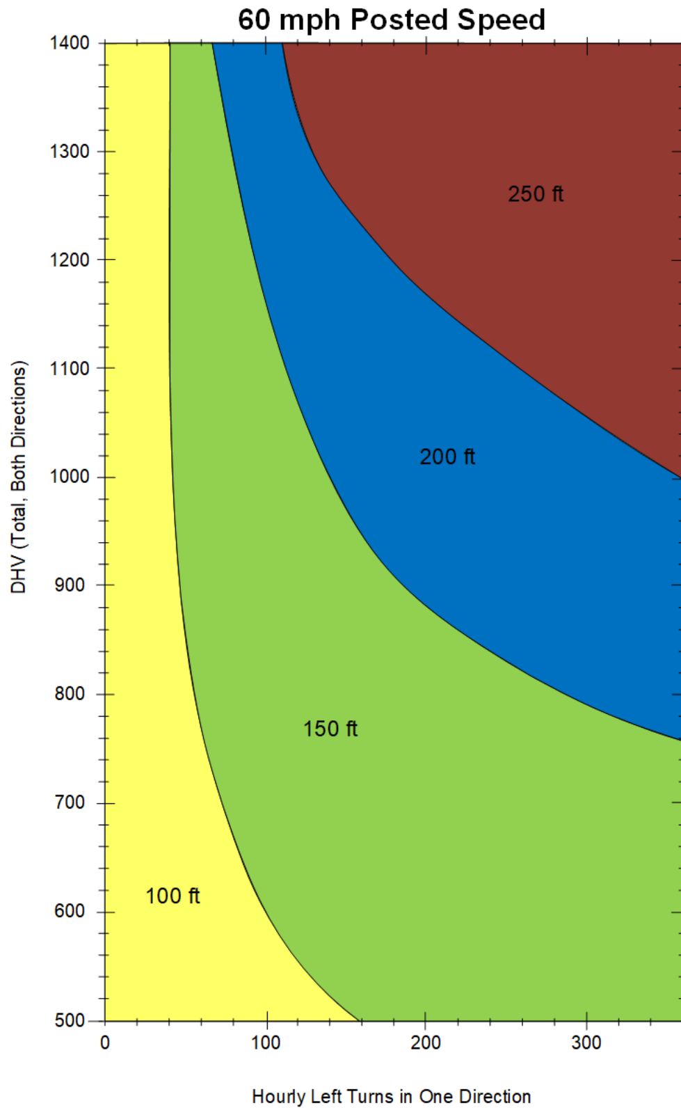
Exhibit 1310-11 Left-Turn Storage Length: Two-Lane, Unsignalized (60 mph)
