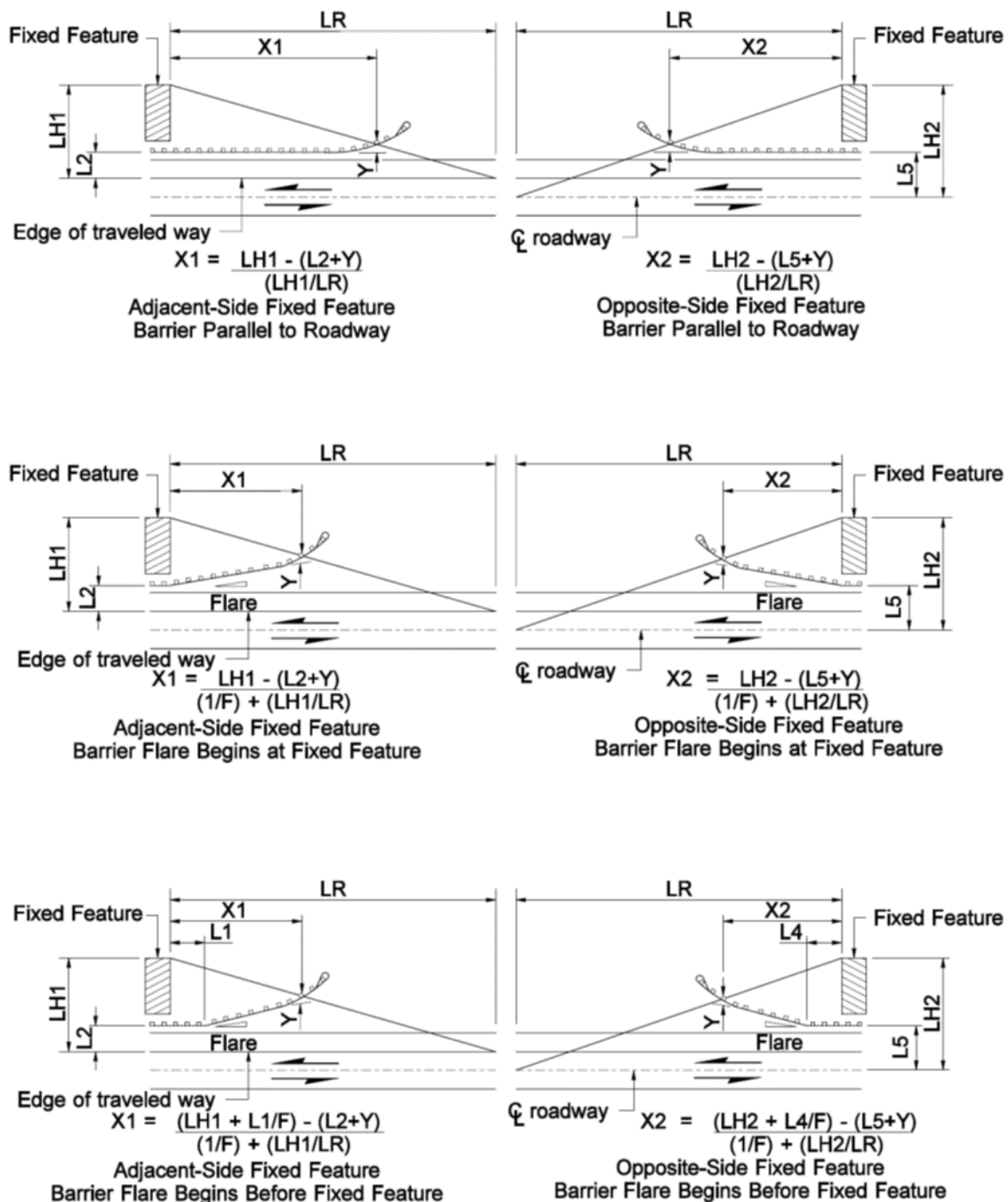
Exhibit 1610-6 Barrier Length of Need on Tangent Sections
