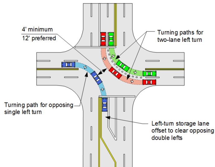
Left-Turn Lane Configuration With Concurrent Phasing
