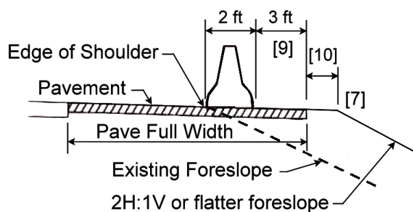
Shoulder Widening for Permanent Barrier (Precast Unanchored Barrier)
