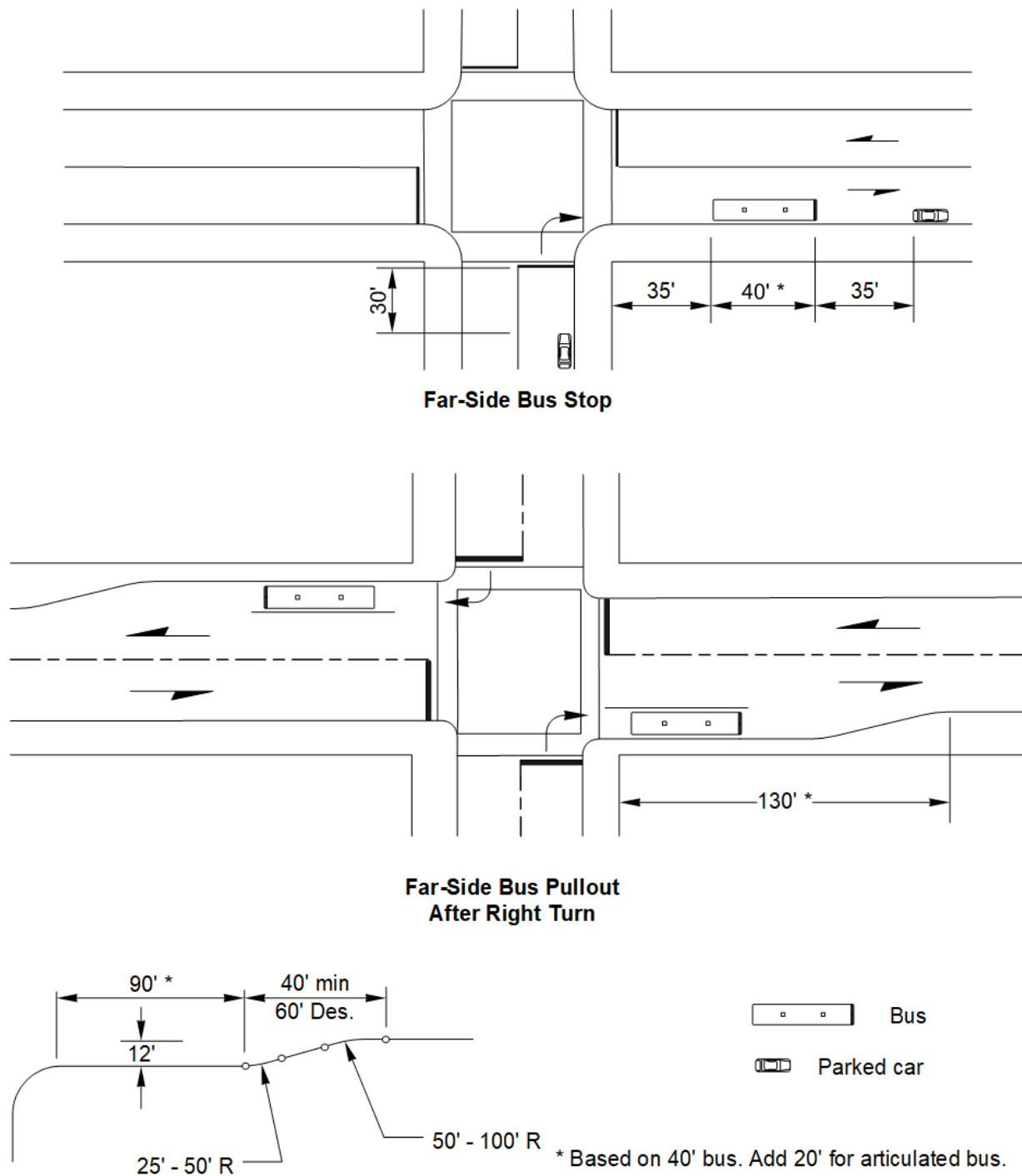
Exhibit 1730-4 Bus Zone and Pullout after Right Turn
