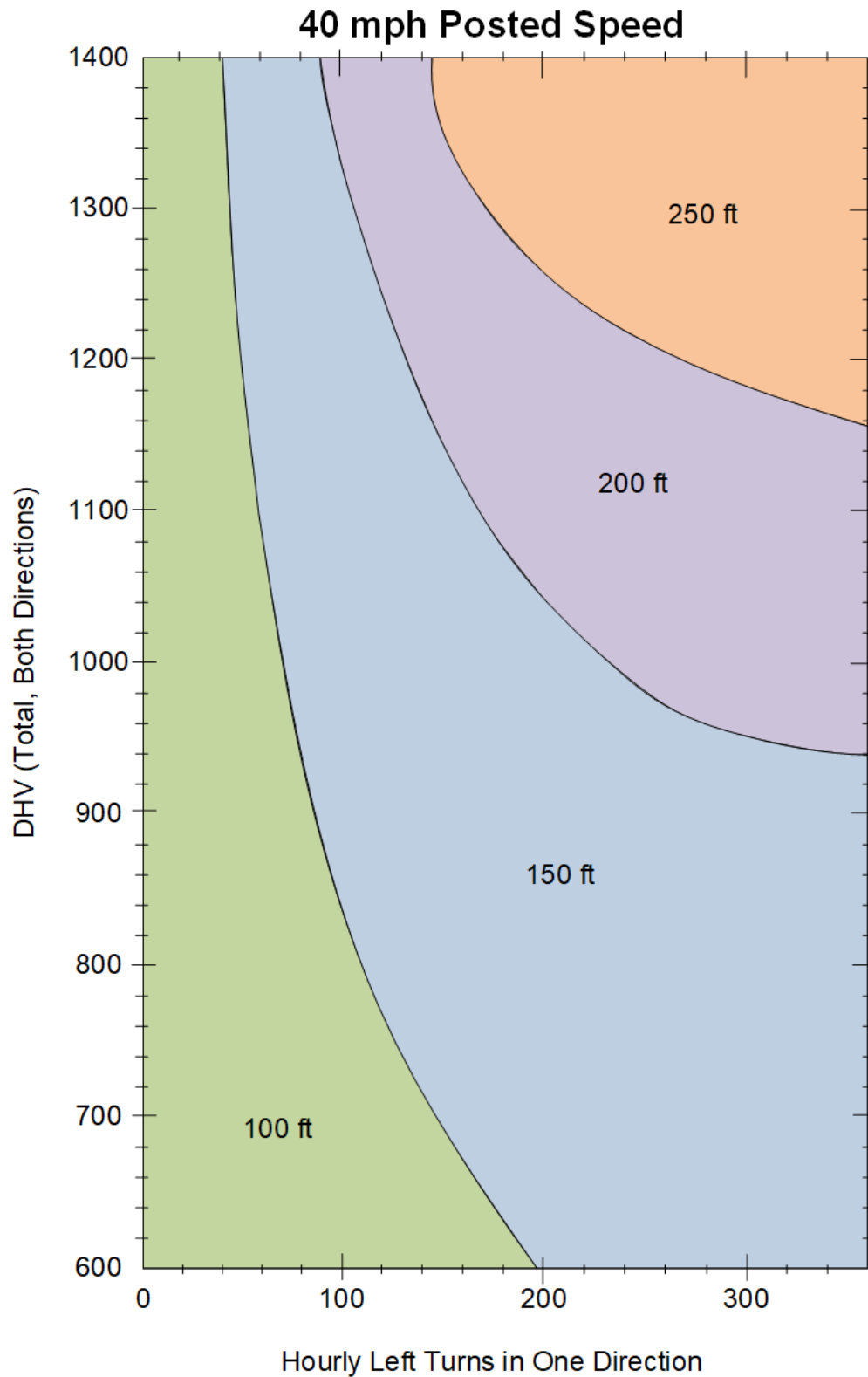
Exhibit 1310-9 Left-Turn Storage Length: Two-Lane, Unsignalized (40mph)
