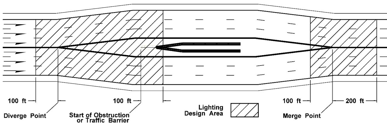
Exhibit 1040-35 Lane Split Lighting Design Area
