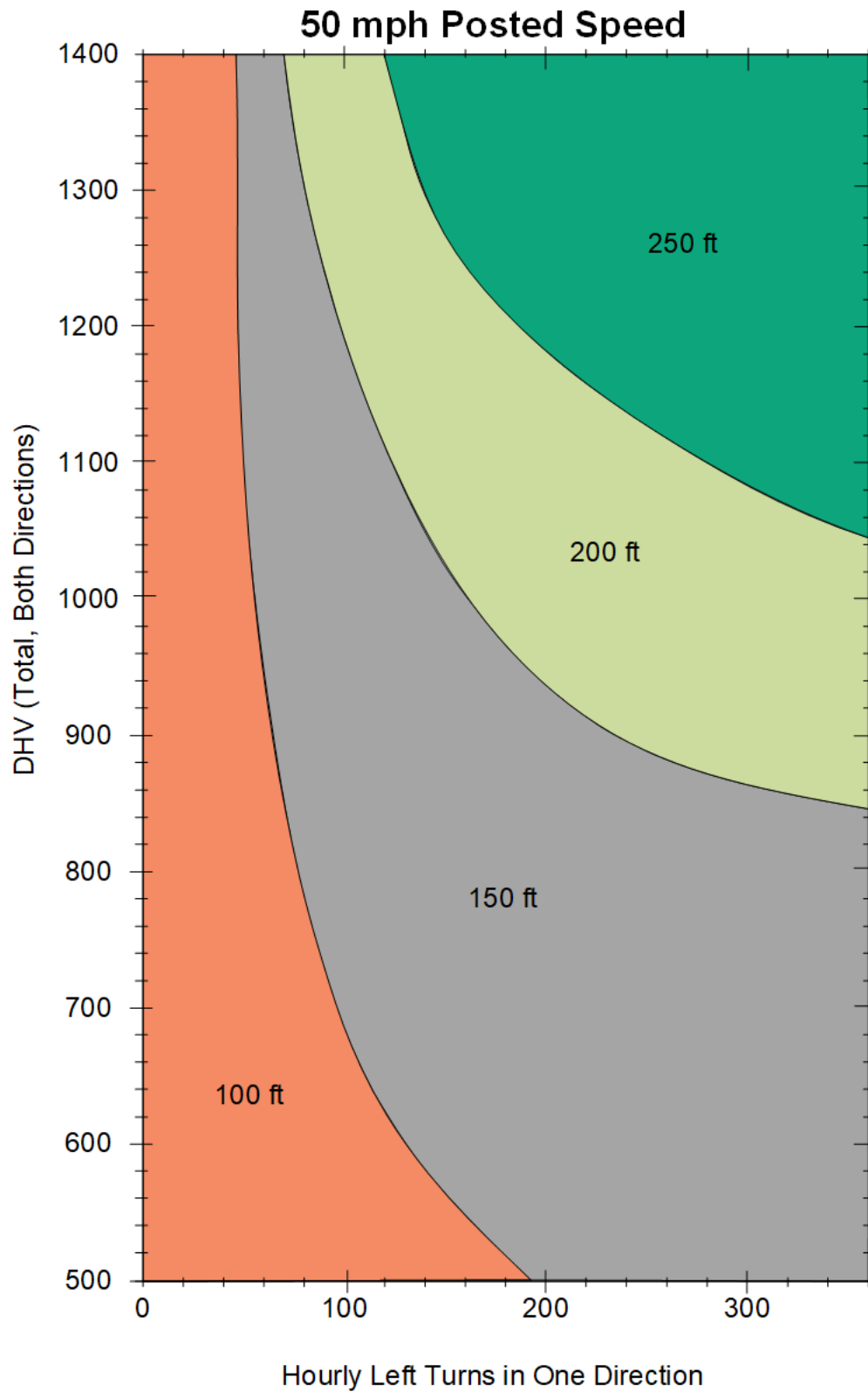
Exhibit 1310-10 Left-Turn Storage Length: Two-Lane, Unsignalized (50 mph)
