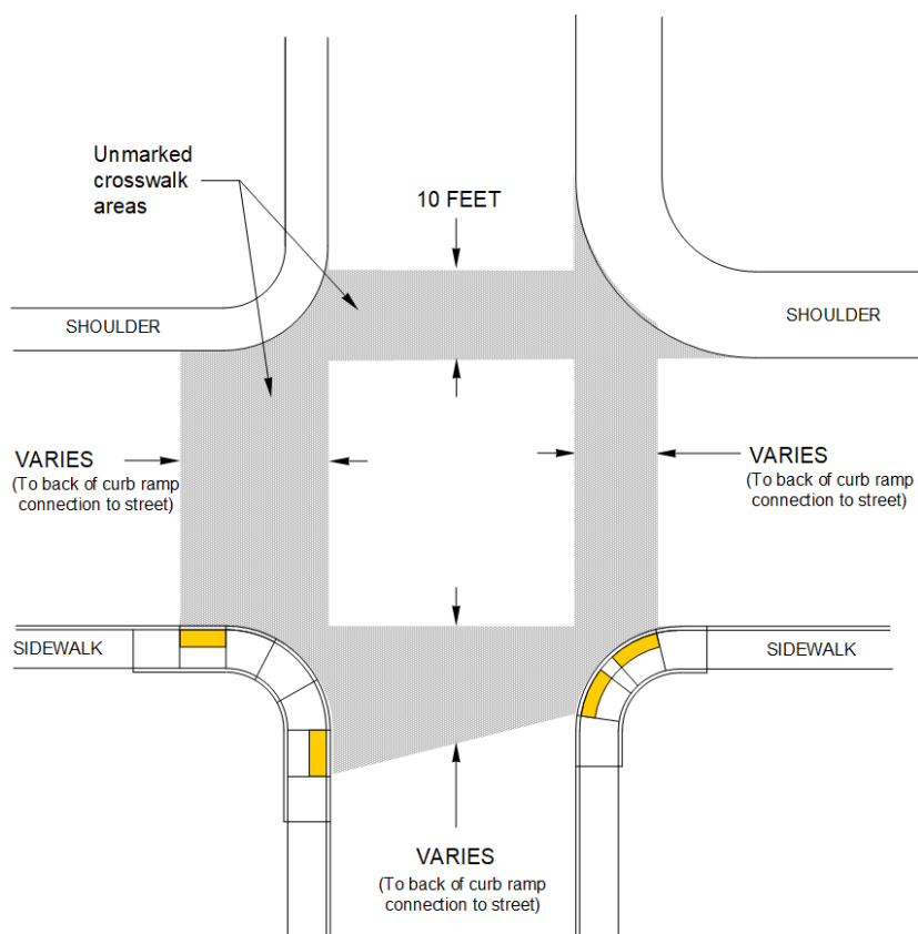
Exhibit 1510-15 Unmarked Crosswalks
