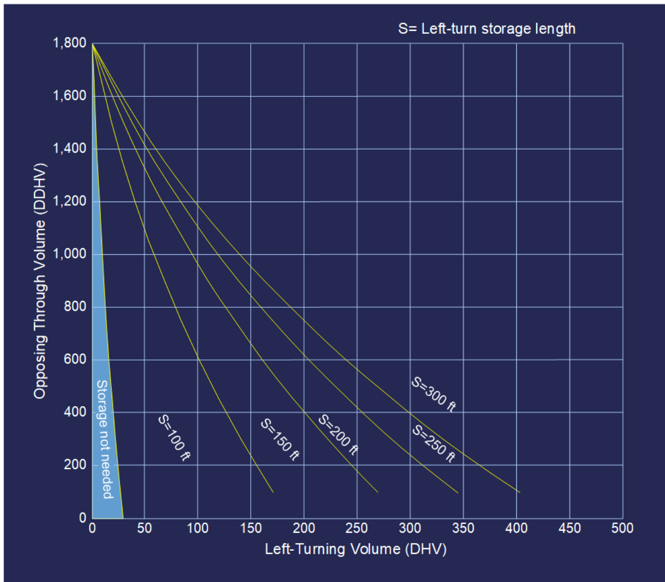
Exhibit 1310-8 Left-Turn Storage Guidelines: Four-Lane, Unsignalized
