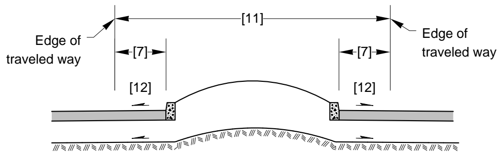
Design F: Raised Median [13]
