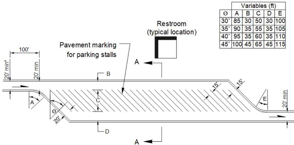
Exhibit 1710-5 Typical Truck Storage
