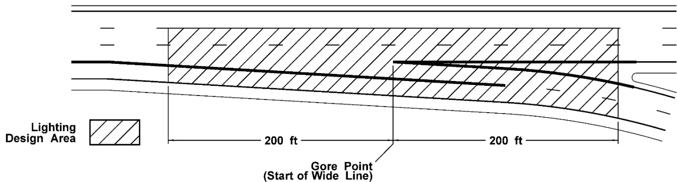
Exhibit 1040-19 Multi-Lane Off-Ramp Lighting Design Area
