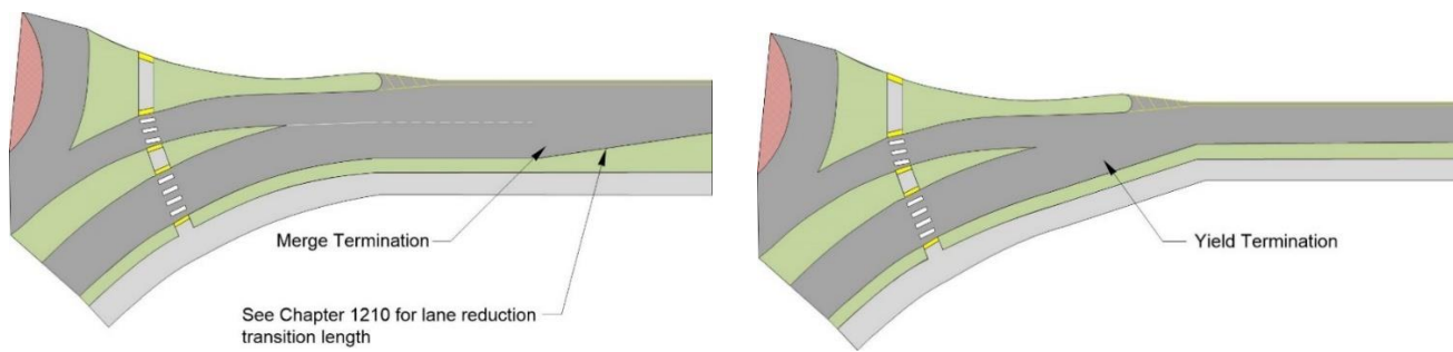
Right-turn slip lanes showing merge and yield termination
