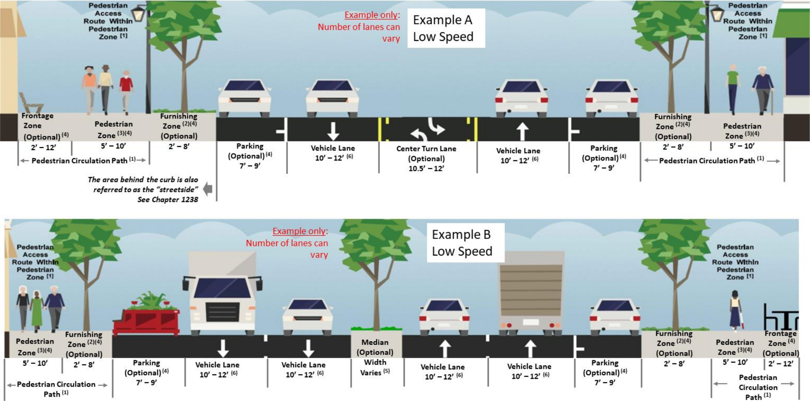
Exhibit 1231-4 Cross Sections Featuring Pedestrian Facilities
