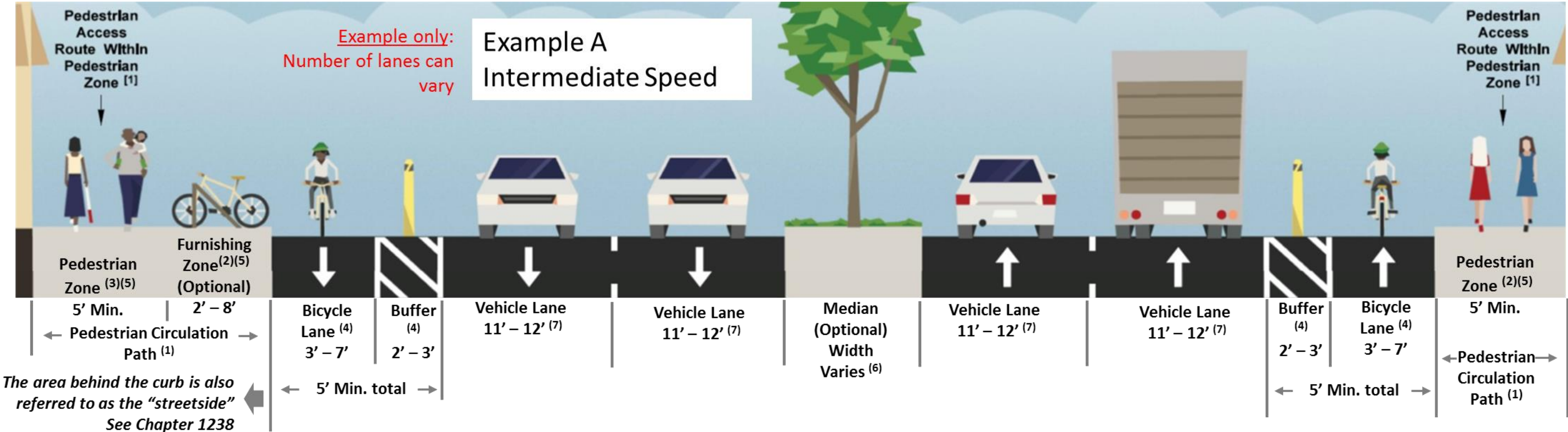
Exhibit 1231-3 Cross Sections Featuring Bicycle Facilities
